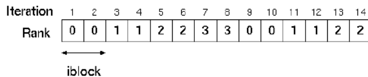
Figure 52. Block-Cyclic Distribution
